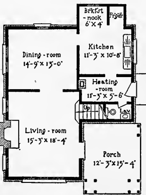
First-floor Plan
